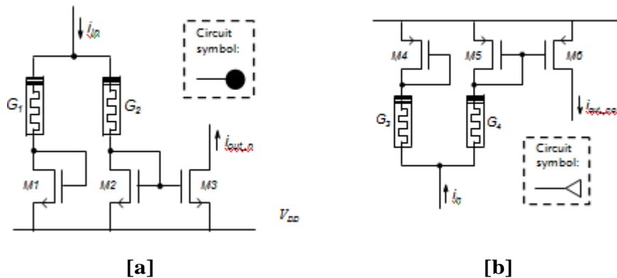
Figure 3: [a] Inhibitory memristive synapse circuit and [b] excitatory memristive synapse circuit. These circuits are inspired by the function of biological inhibitory (e.g. GABAergic) and excitatory (e.g. glutamatergic) synapses with ionotropic receptors
