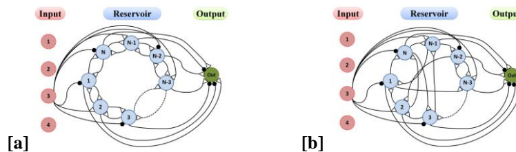
Figure 2: Block level representations of the two ESN topologies that can be embedded in the proposed architecture.[a] Ring topology and [b] Random topology. All the simulations for the hardware architecture are performed with random topology.
