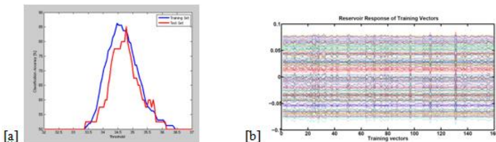
Figure 5: [a] The accuracy of detecting the epileptic seizure using the limited-precision ESN hardware architecture. The maximum test accuracy is 85%. [b] ESN reservoir response to all of the training vectors.
