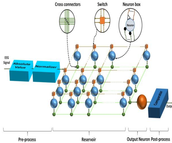
Figure 1: High-level depiction of the ESN architecture. The core reservoir is based on the cellular automata architecture with reconfigurable crossconnectors, enabling dynamic configuration of different ESN topologies. The output node is implemented using bi-stable memristive synapses.
