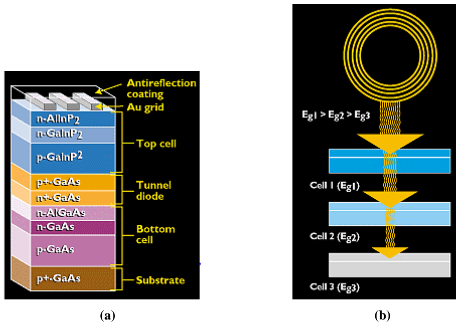
Fig.1 Multi-junction of a Photo-voltaic cell. (a) Structure (b) photon absorption [1]
