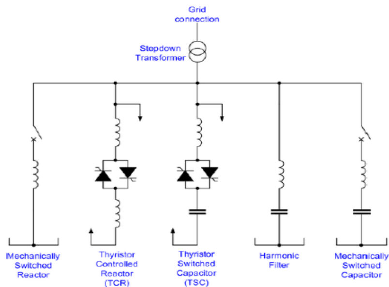
Fig.1 A typical SVC Configuration
