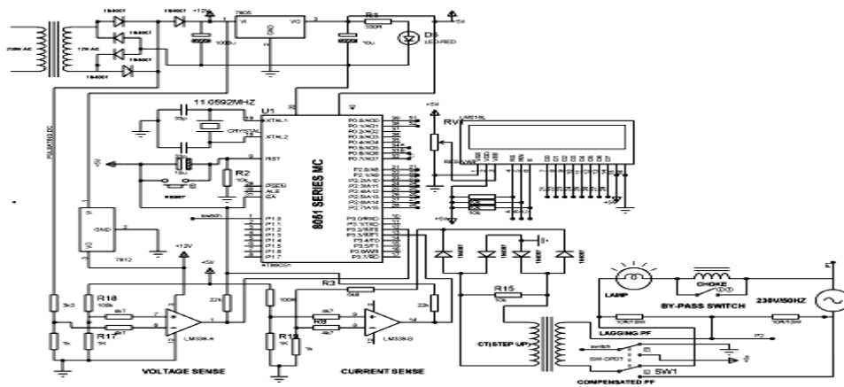
Fig.4. Hard ware component diagram of compensated power system
