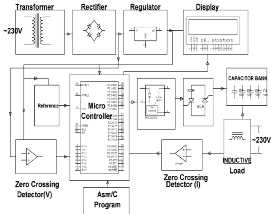
Fig.2. Block diagram of single-phase SVC with R-L load
