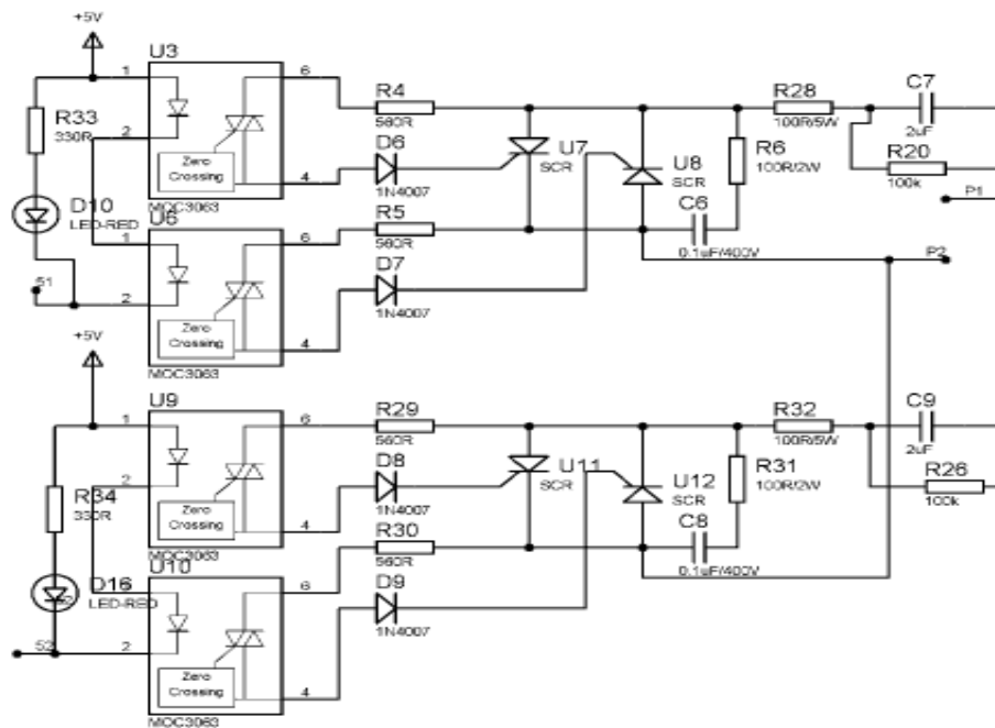
Fig.3. Switching and converter circuit
