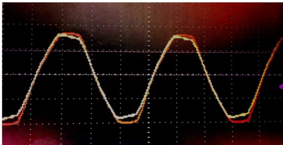
Fig.6. voltage and current waveform without compensation with R-load
