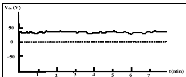
Fig. 4. The DC voltage measured across each PV unit (12 V DC)
