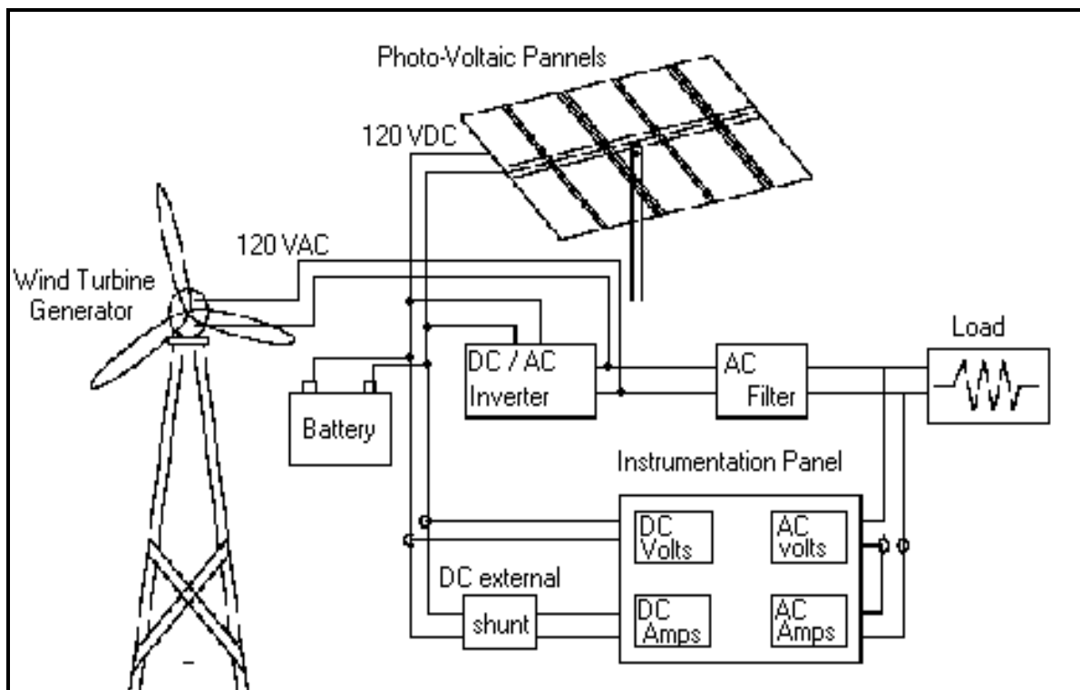
Figure 3 A simple Hybrid Solar & Wind System Methodology
