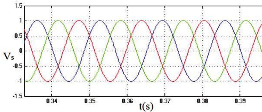
Fig.4 Source Voltage (pu) Waveforms of the System
