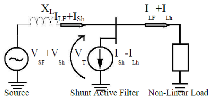
Fig.2 Principle of Shunt Current Compensation
