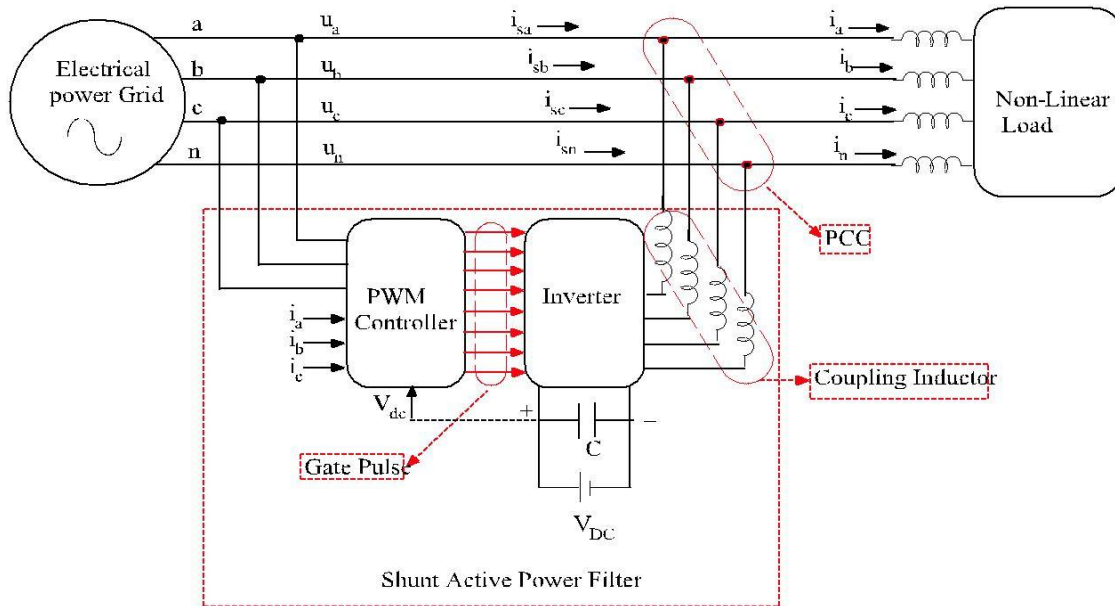
Fig.1 Shunt active power filters topology.
