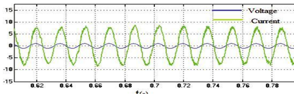
Fig.10 Power Factor Improvement Using PI Controller
