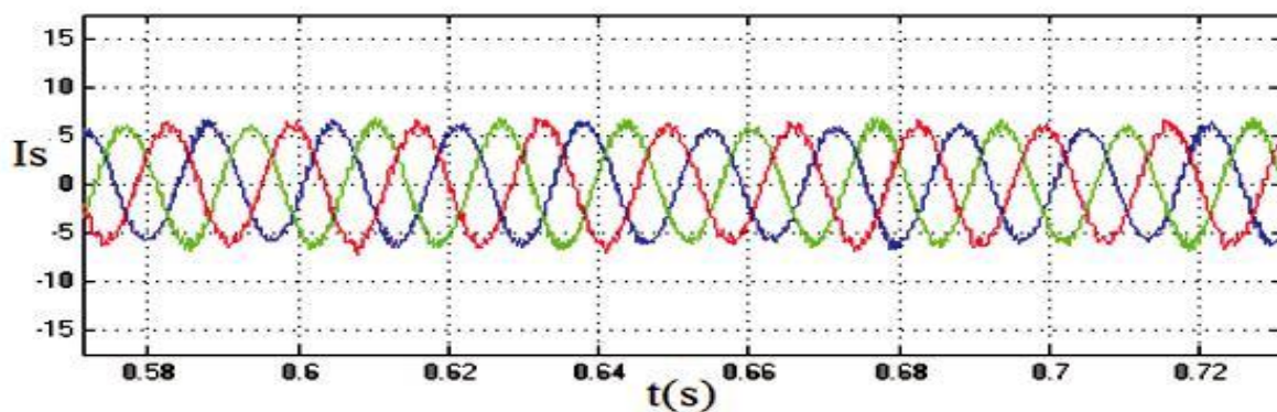
Fig.6 Compensating Current of PI Controller.
