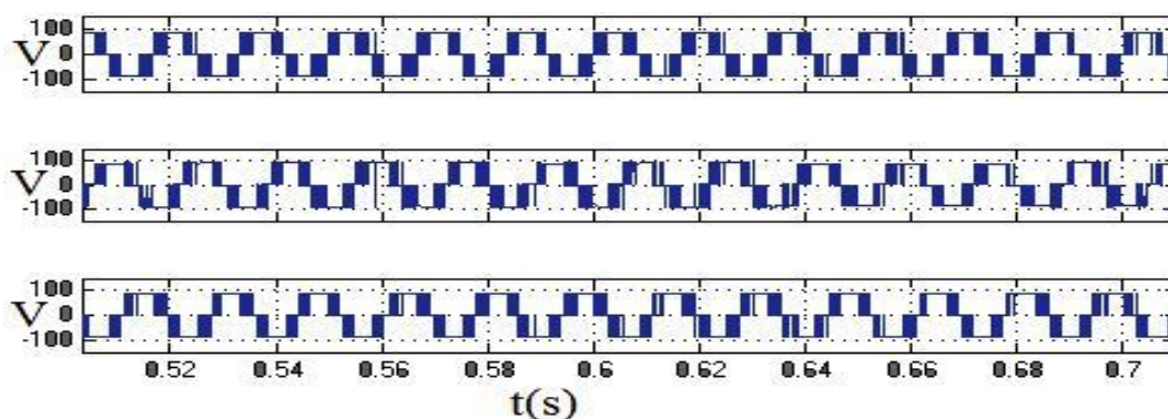
Fig.12 Three phase Voltage Generated by APF
