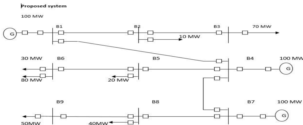
Fig.No.1.Proposed 9-bus system
