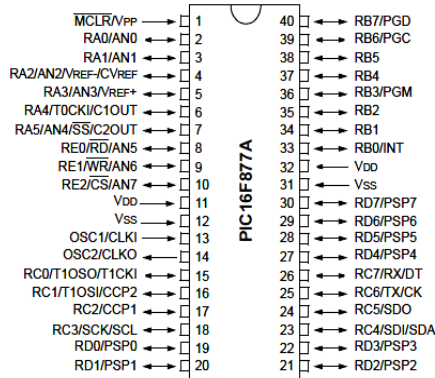
Fig. 5 Pin diagram of PIC16F877A microcontroller
