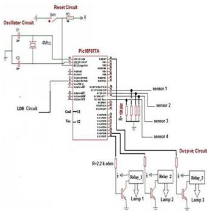
Fig. 7 Schematic circuit of the street light system
